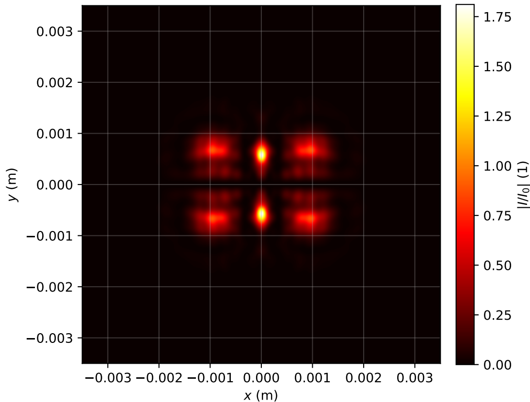
Intensity profile I(x, y, z = 1.194)/I_0 , \text{Pin}=8.0\text{Pcr} , artificial time
